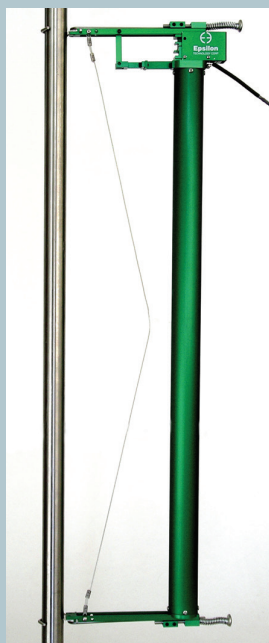
Model 3542L with 500 mm gauge length and +10 mm/-6 mm measuring range
